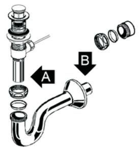
Typical Drain Assembly
